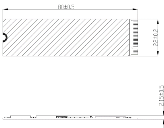
<Without heatsink>
