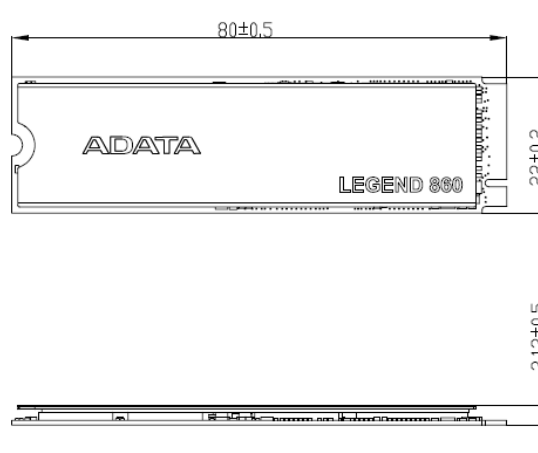
<With heatsink>
