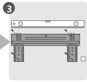
Attach mounting plate
