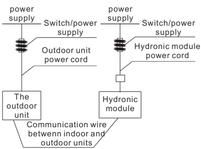
Figure 5-1 Wiring and Control
