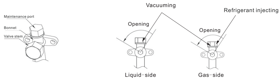
Figure 4-4 Illustration of the shut-off valve
