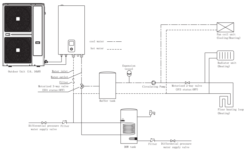
Figure 3.7 Cooling Mode operation
