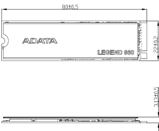
<With heatsink>
