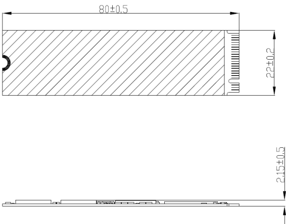
<Without heatsink>
