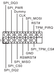
SPI_TPM_J1
