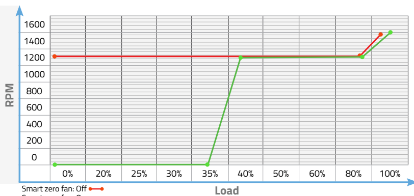
Load vs RPM
