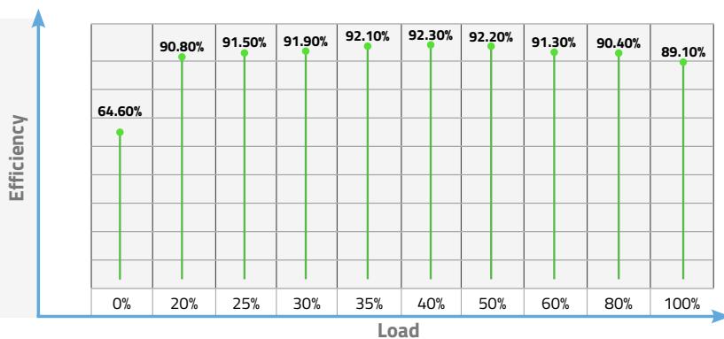
Load vs Efficiency
