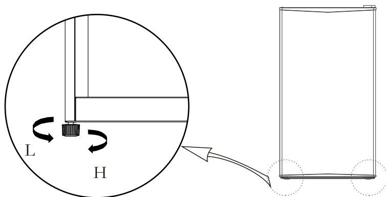
Schematic diagram of the levelling feet
