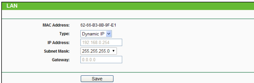
Figure 4-6 LAN – Smart IP (DHCP)
