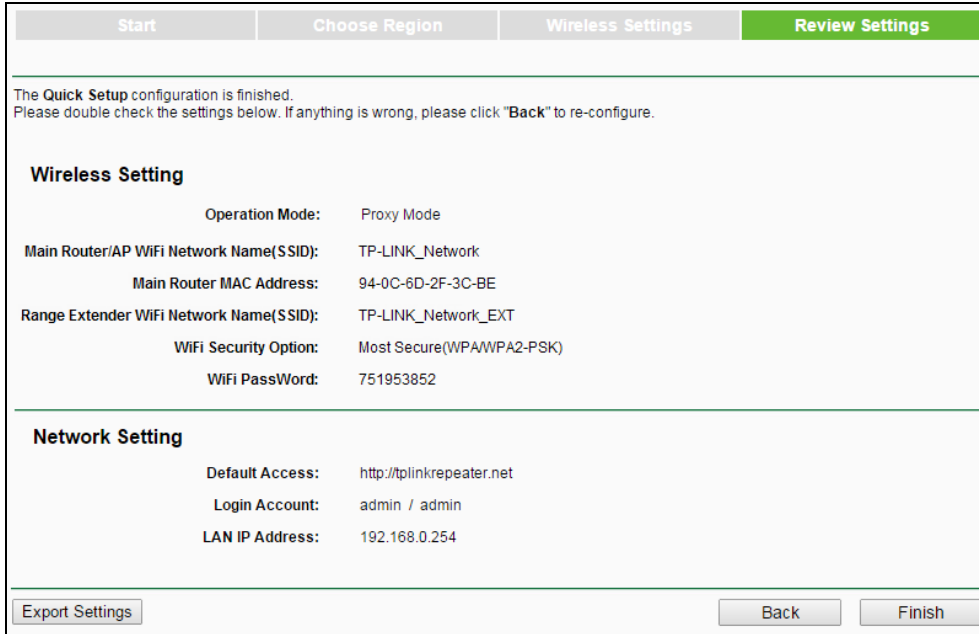
Figure 3-8 Quick Setup – Review Settings
