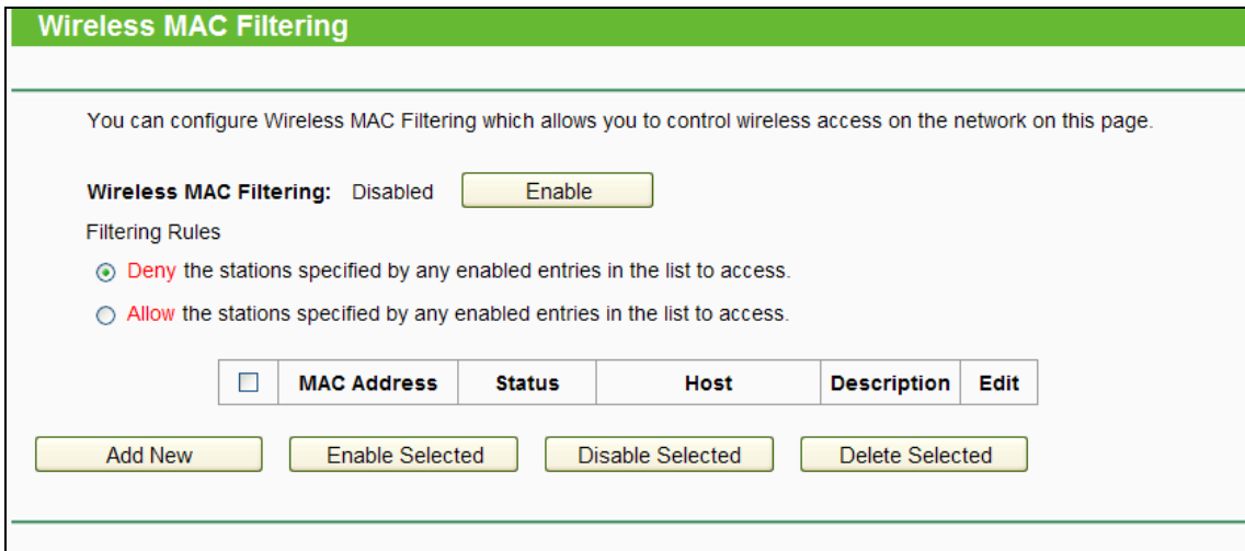
Figure 4-25 Wireless MAC Filtering
