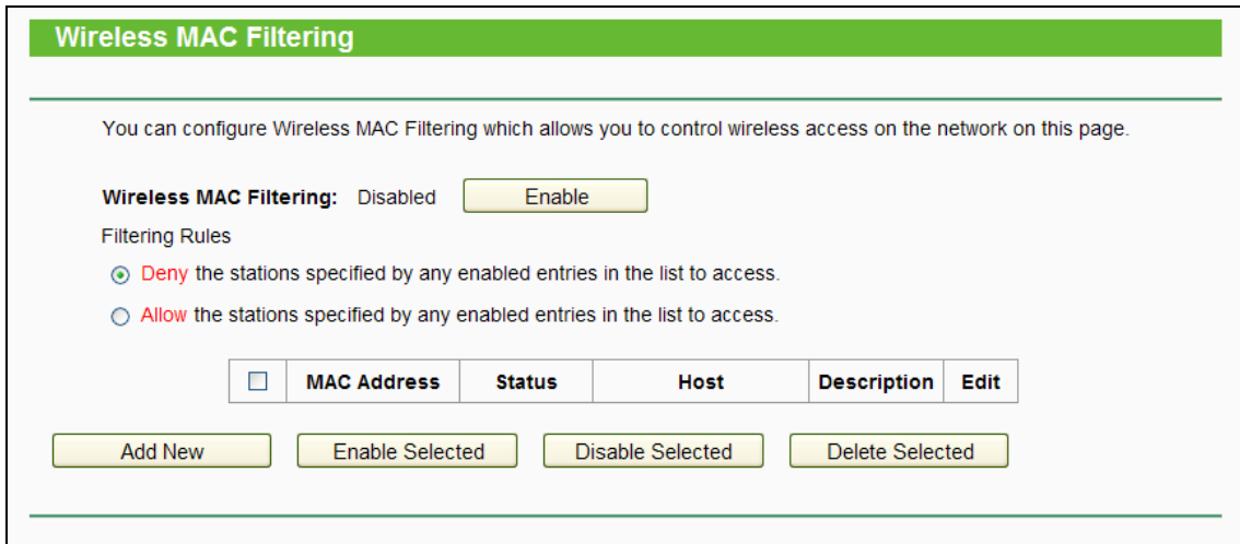
Figure 4-40 Wireless MAC Filtering
