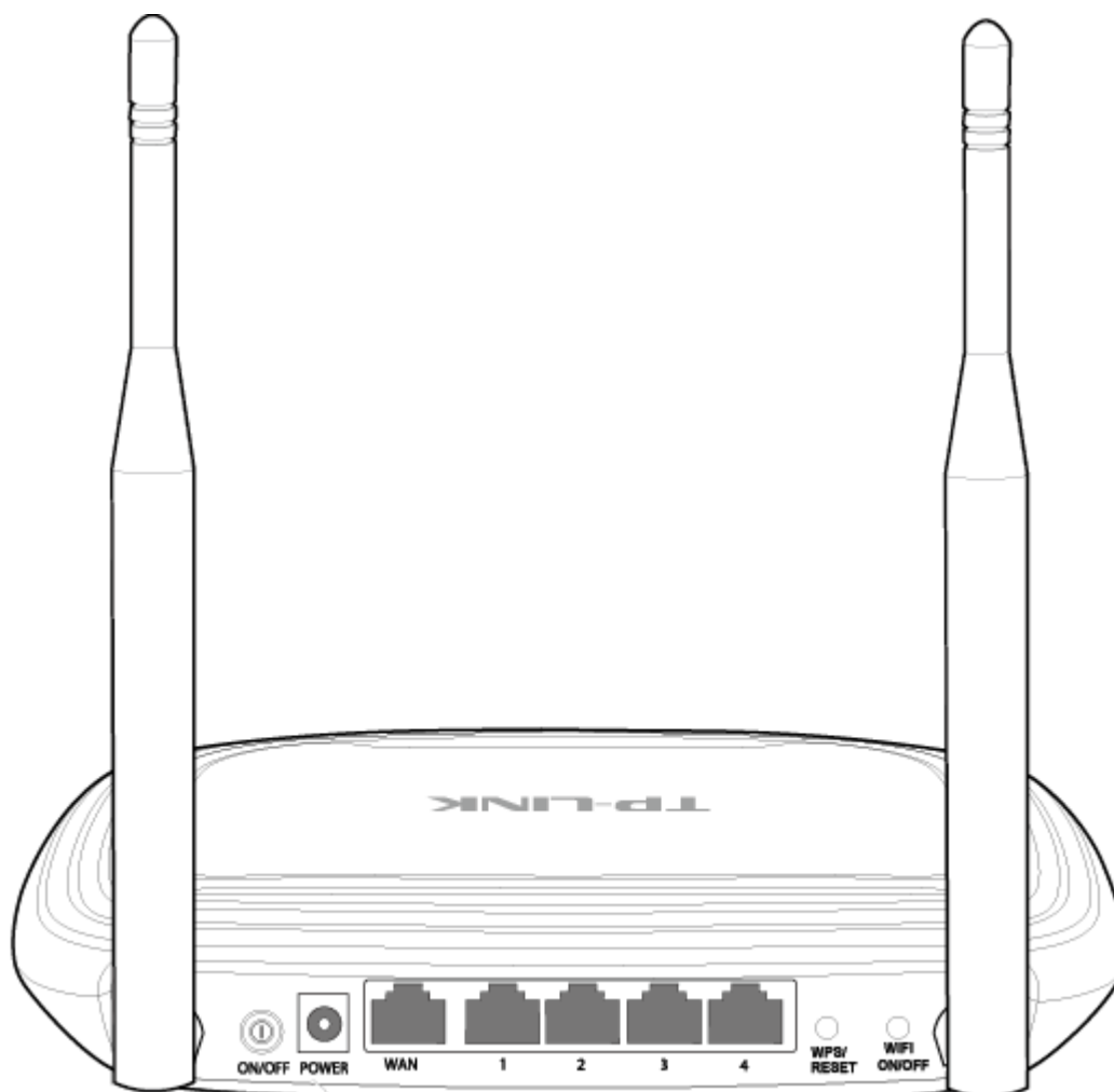
Figure 1-2 Rear Panel sketch
