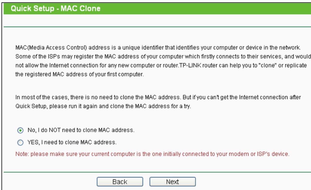
Figure 3-7 MAC Clone
