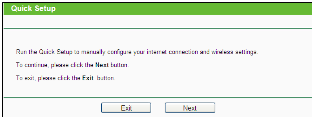
Figure 3-5 Quick Setup
