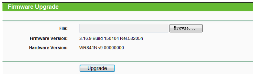
Figure 4-76 Firmware Upgrade
