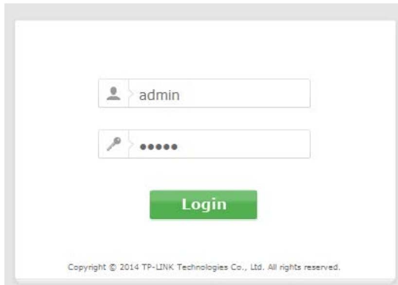
Figure 3-4 Login Windows
