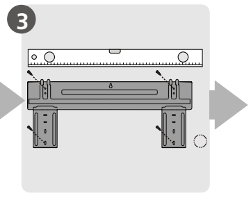
3 Attach mounting plate
