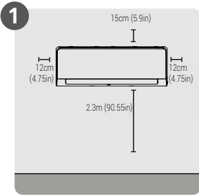
1 Select installation location
