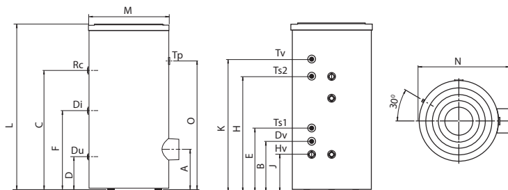
Model 200-1, 300-1
