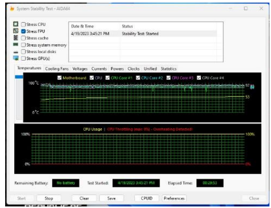
AIDA64 Extreme
