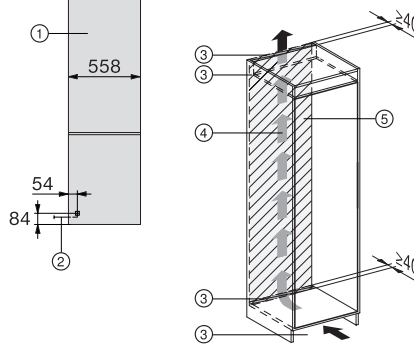
KFN7714F, KFNS7716FC, installation (footnote*) (installation drawings)
