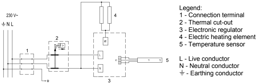
Fig. 6: Electric installation
