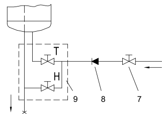
Fig. 4: Open (non-pressure) system
