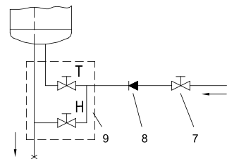
Abb. 4: Offenes System (druckloses System)
