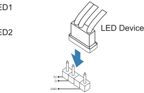
Addressable RGB LED Device Header (5V_LED)
