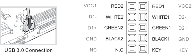
USB 3.0 Connection
