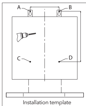
Installation template
