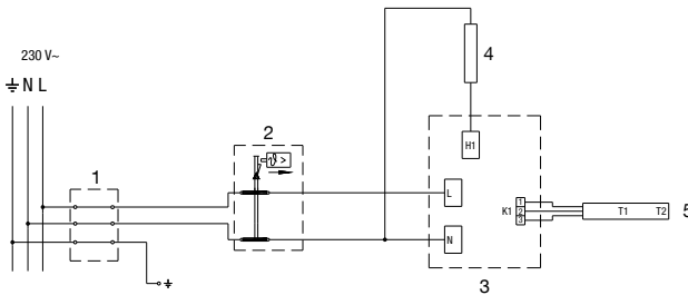
Fig. 5: Electric installation
